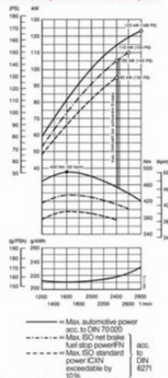
Power, torque and fuel consumption
