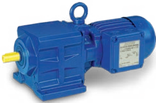
Helical Gear Motor Series BG Bauer Gear Motor
