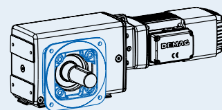
WF flange-mounting
